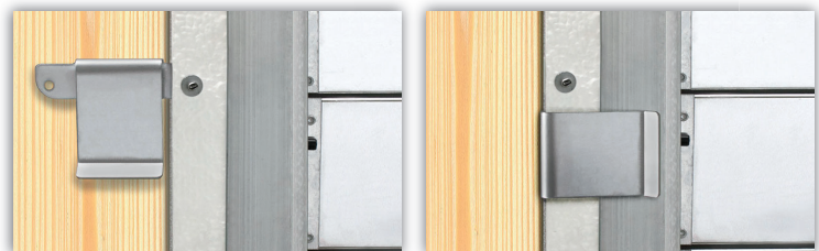
Stainless steel heavy gauge shutter clips swivel by hand for easy removal of the shutter when it's time to clean or maintain your fan.
